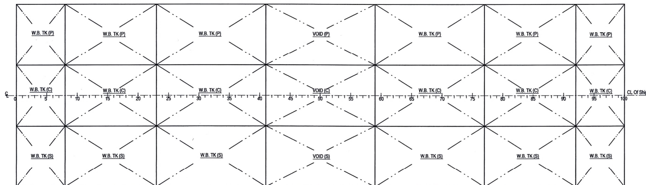
BELOWDECK PLAN
